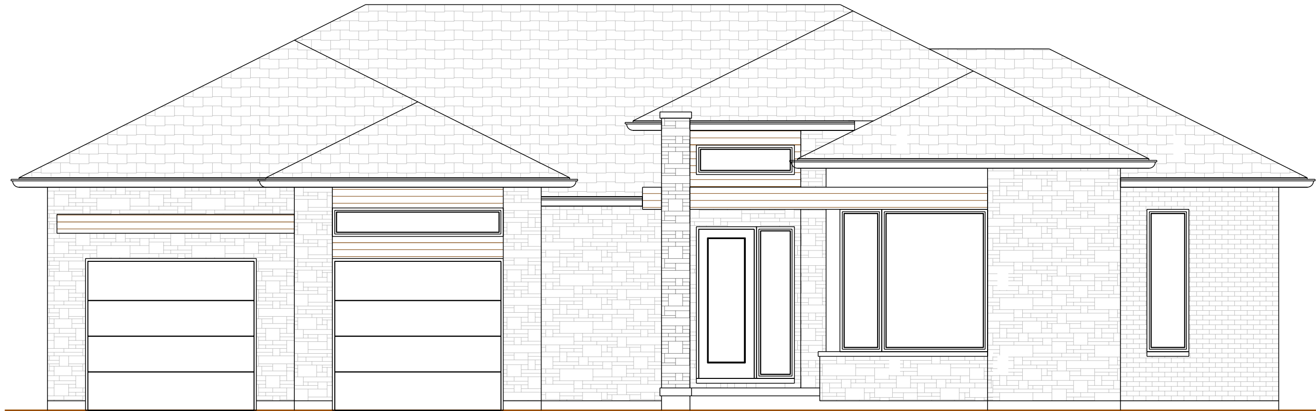
3B ELEVATIONS PRO MATERIAL SCALE: 1" = 5'-0"
